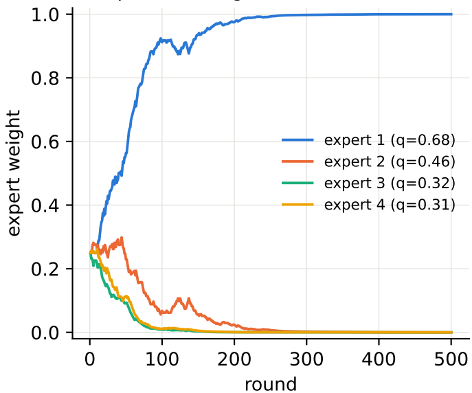
Multiplicative weights (exact)
