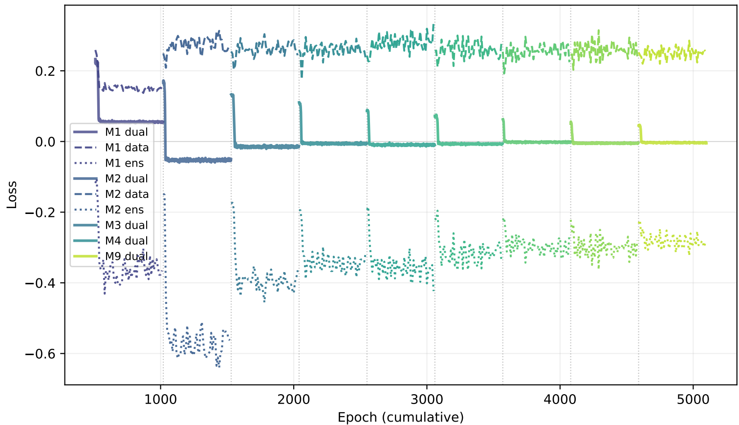
Dual MMD Losses ( \hat{\text{data}} , v ensemble)
