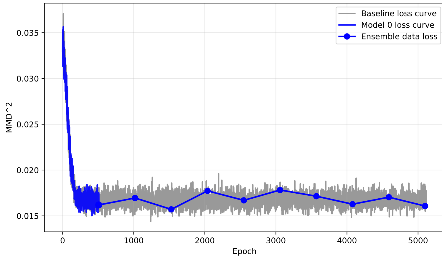
Ensemble MMD 2 vs Data
