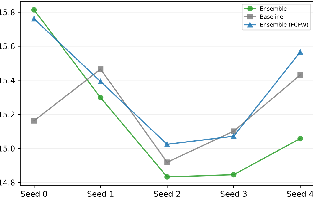
training_loss
