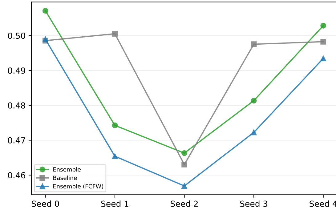
mmd
