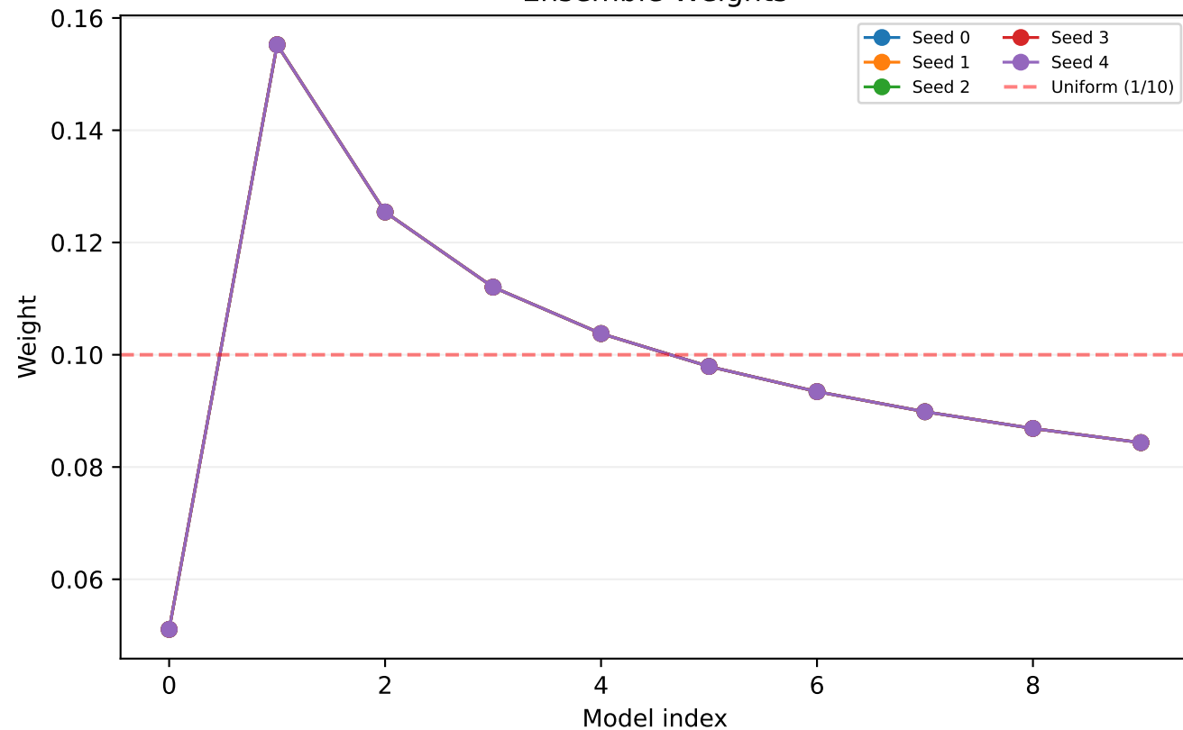
Ensemble Weights
