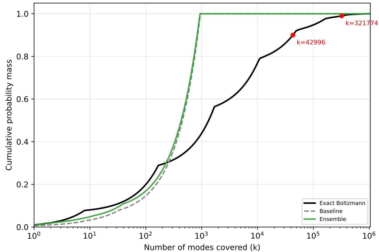
Lorenz curve
