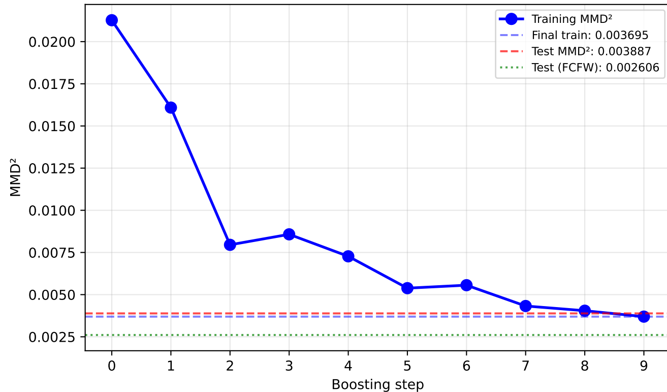
MMD 2 Progression (Trial 14)
