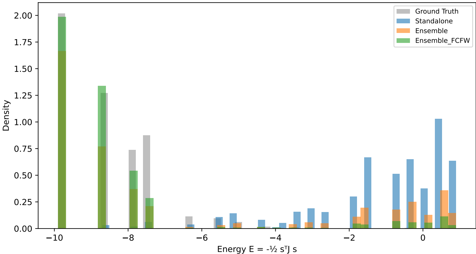
Hopfield energy distribution
