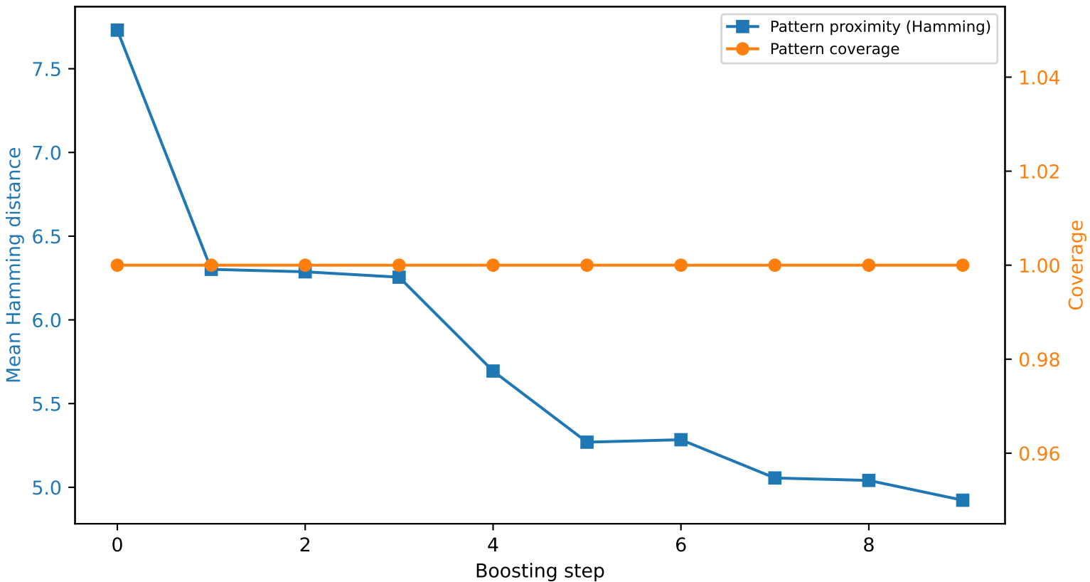
Hopfield — incremental ensemble proximity & coverage
