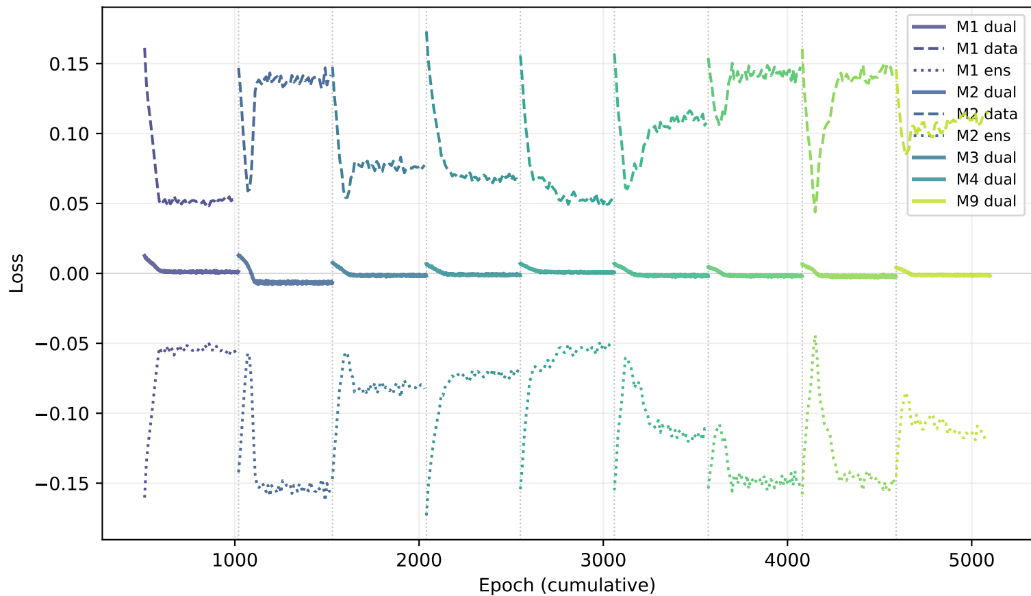
Dual MMD Losses ( \hat{\mu} data, v ensemble)
