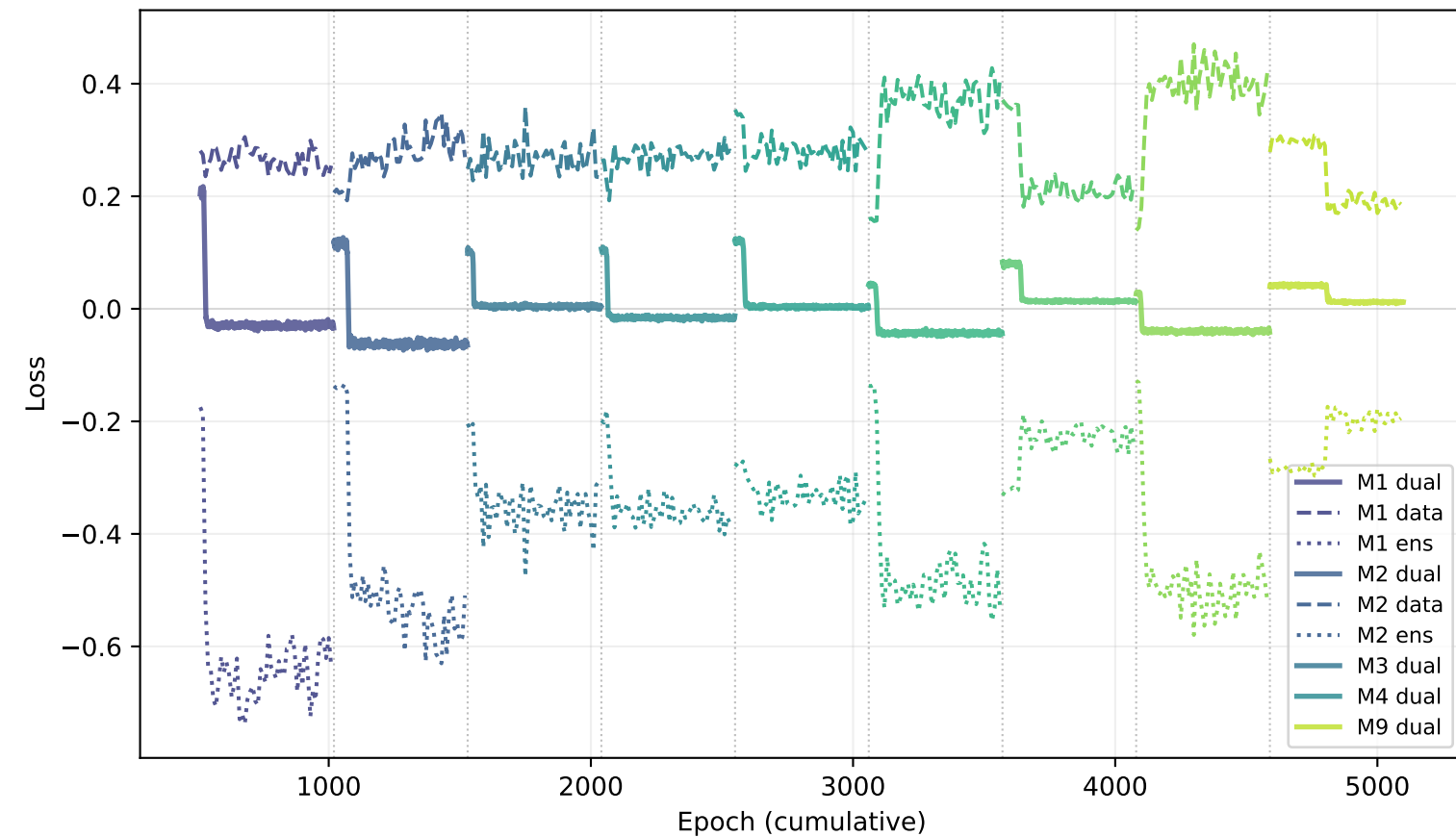
Dual MMD Losses ( \wedge data, v ensemble)
