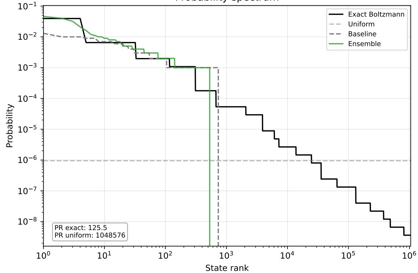
Probability spectrum
