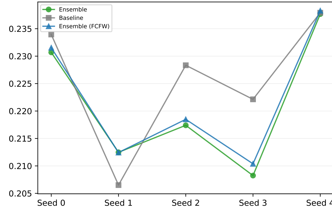
mmd
