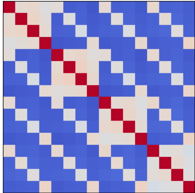
Ground Truth
