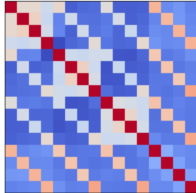
Ensemble_FCFW
