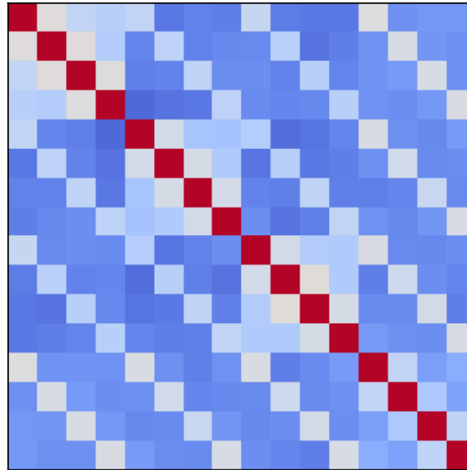
Ensemble
