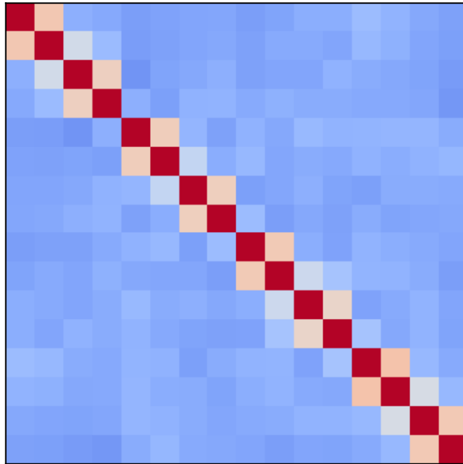
Standalone
