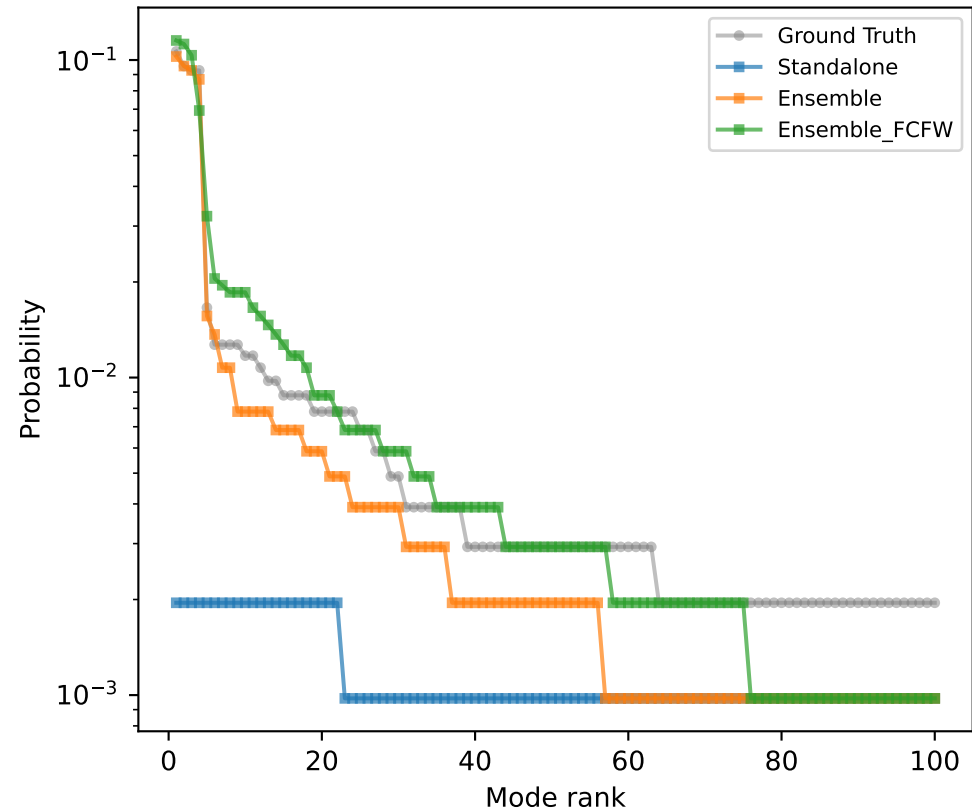
Probability spectrum (top 100 modes)
