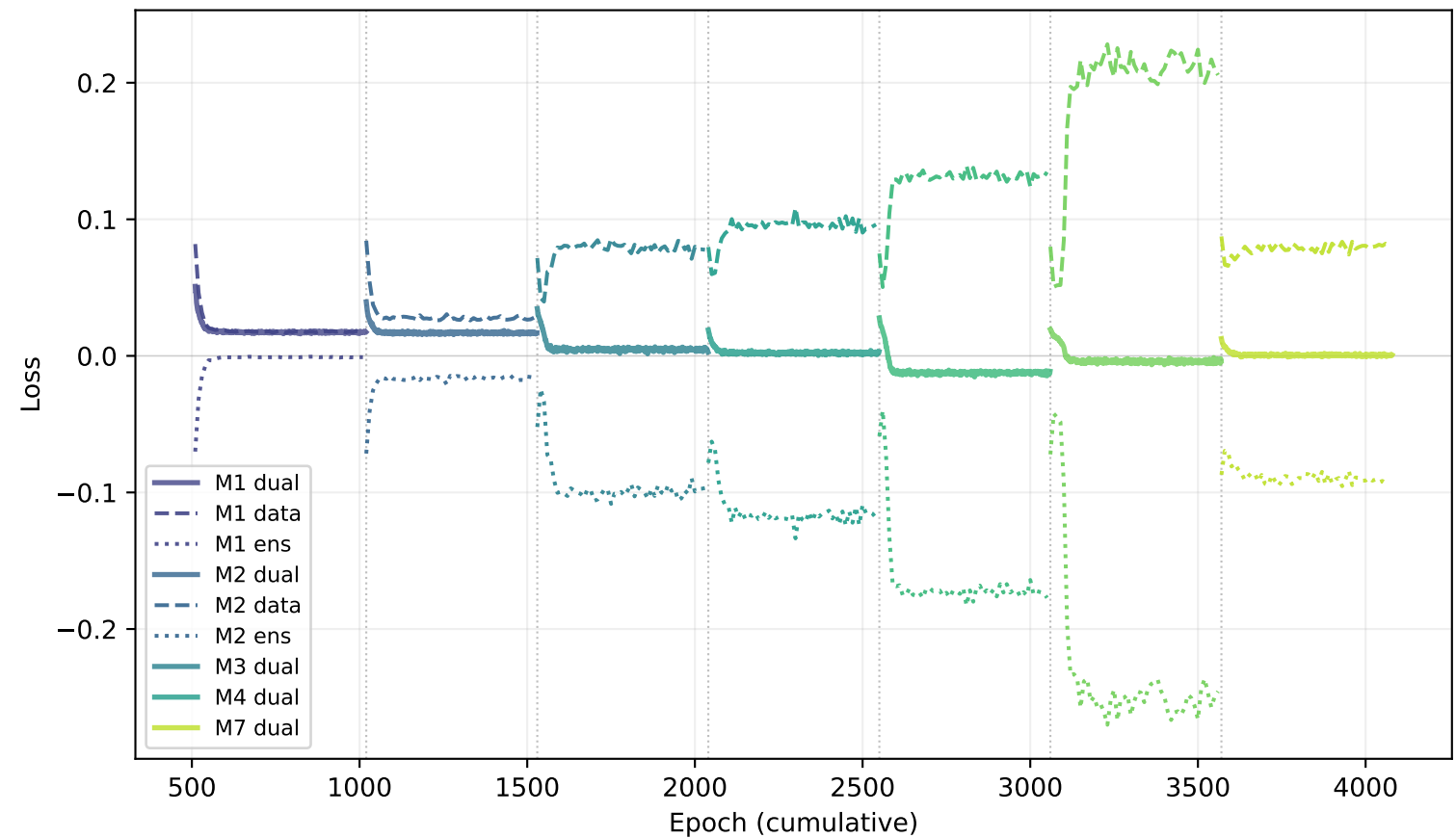
Dual MMD Losses (^ data, v ensemble)
