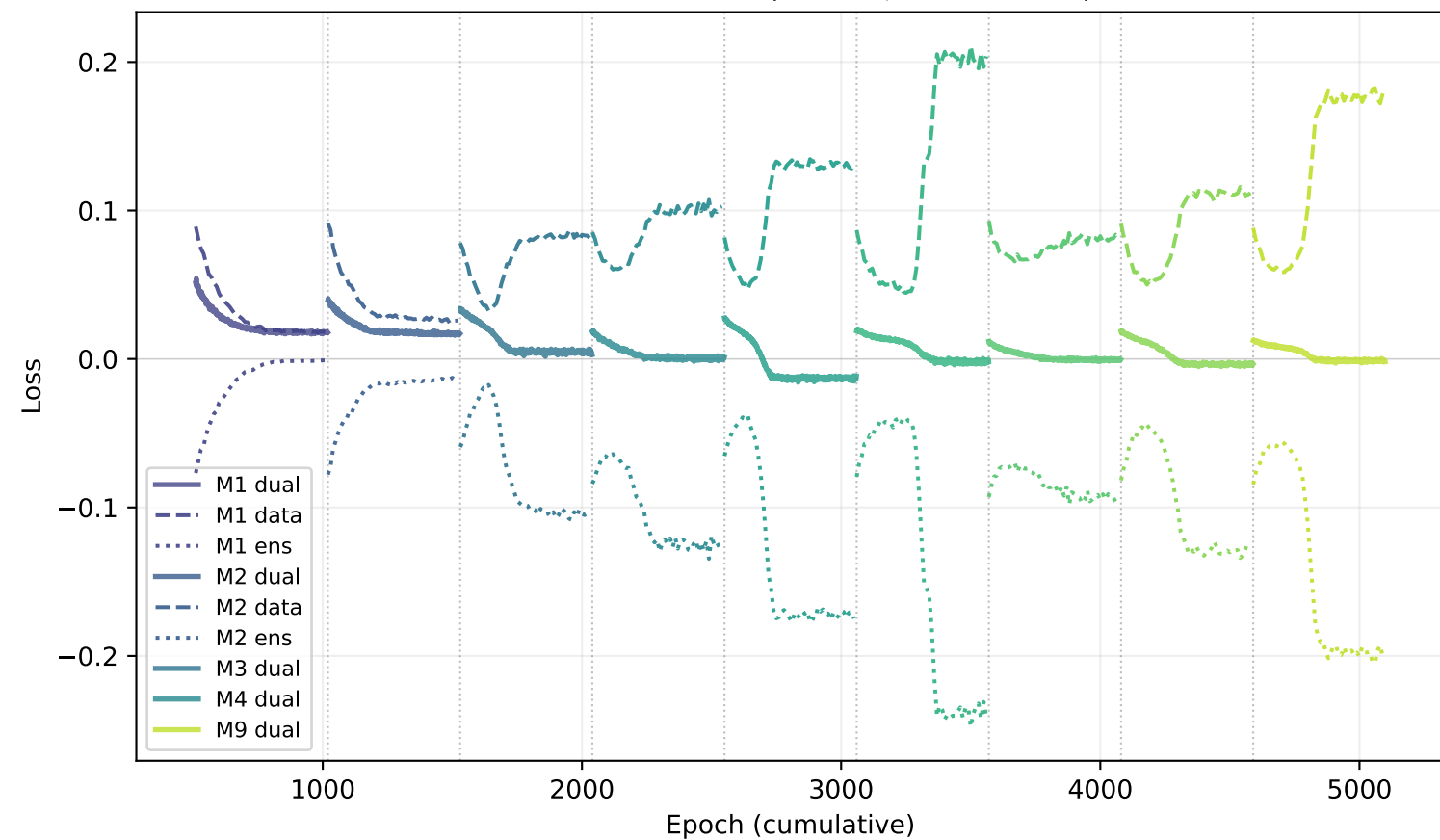
Dual MMD Losses (^ data, v ensemble)
