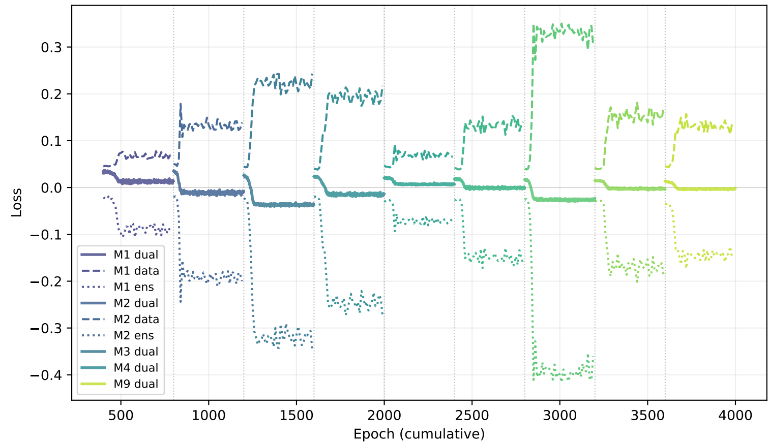
Dual MMD Losses ( \hat{\mu}_{data} , \nu_{ensemble} )
