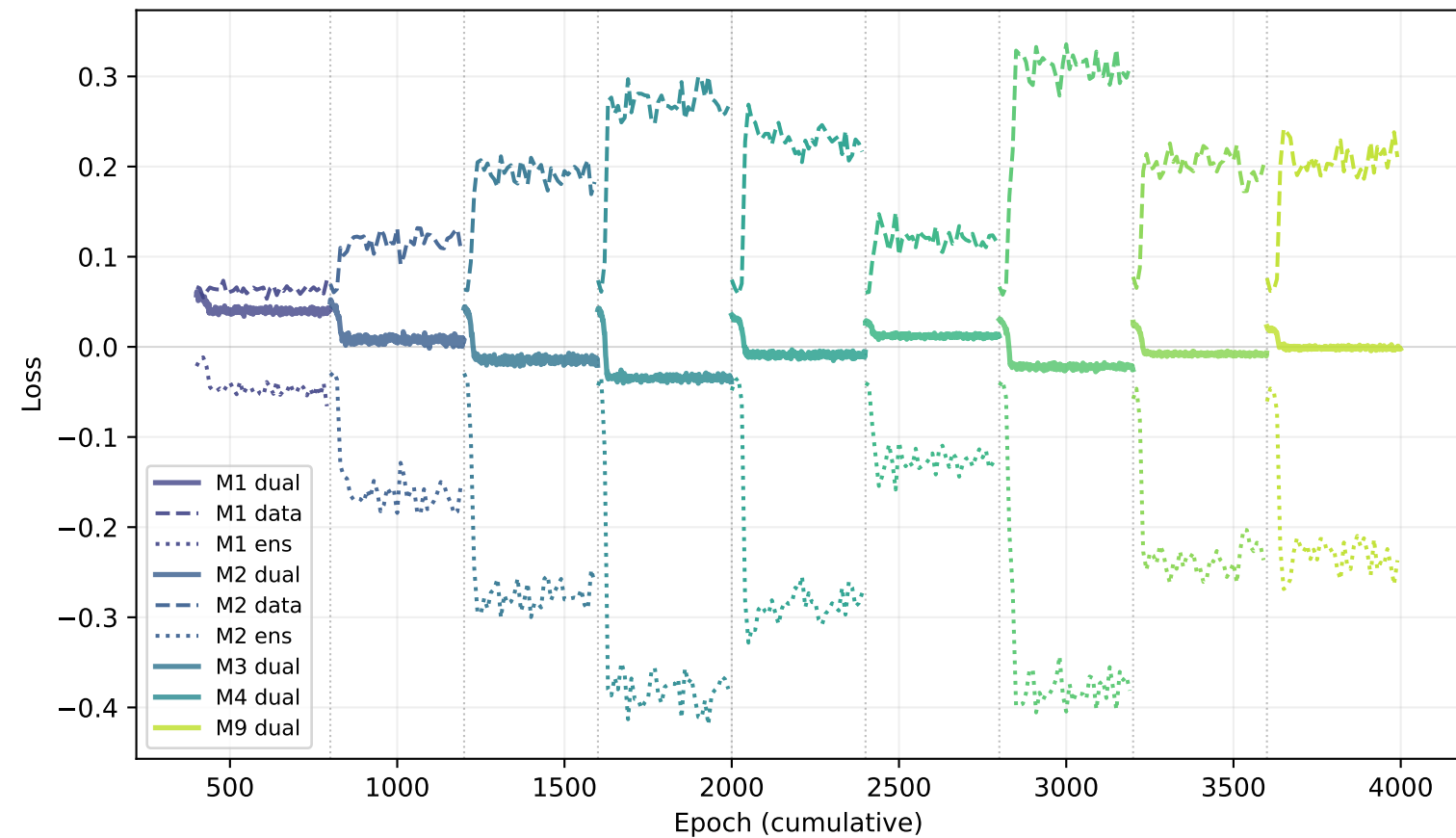
Dual MMD Losses ( \hat{\cdot} data, v ensemble)
