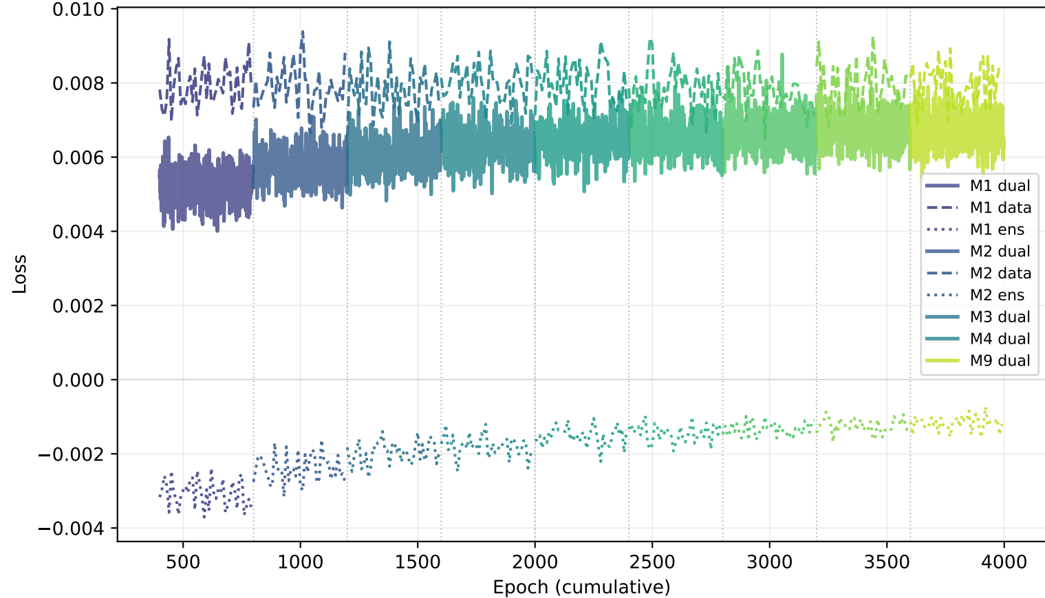
Dual MMD Losses ( \hat{\mu} data, v ensemble)
