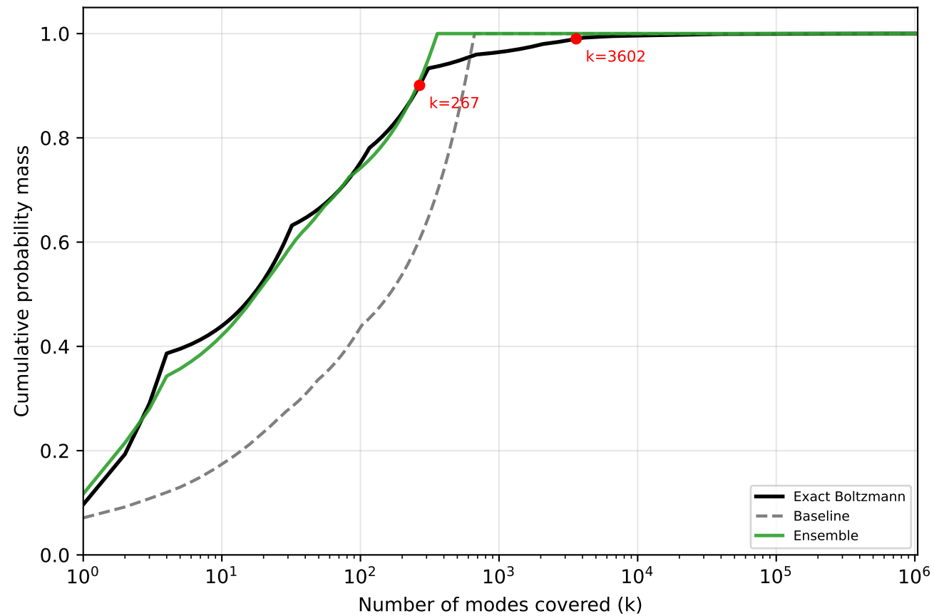
Lorenz curve
