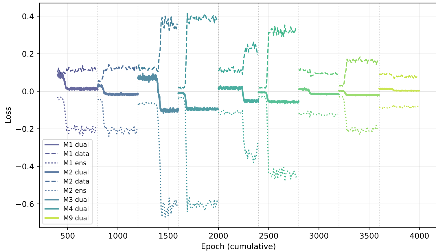
Dual MMD Losses ( \wedge data, v ensemble)
