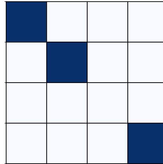
Model 2 | sample 42
