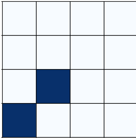
Model 1 | sample 26
