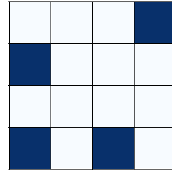
Model 1 | sample 77
