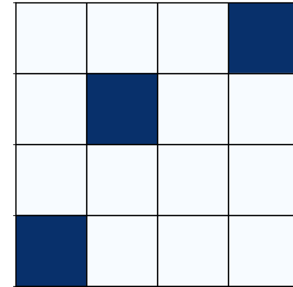
Model 2 | sample 1
