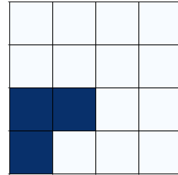
Model 2 | sample 1
