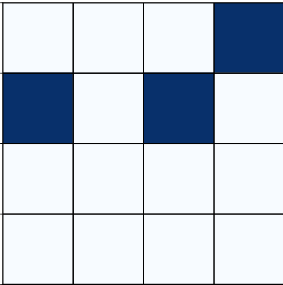
Model 2 | sample 104
