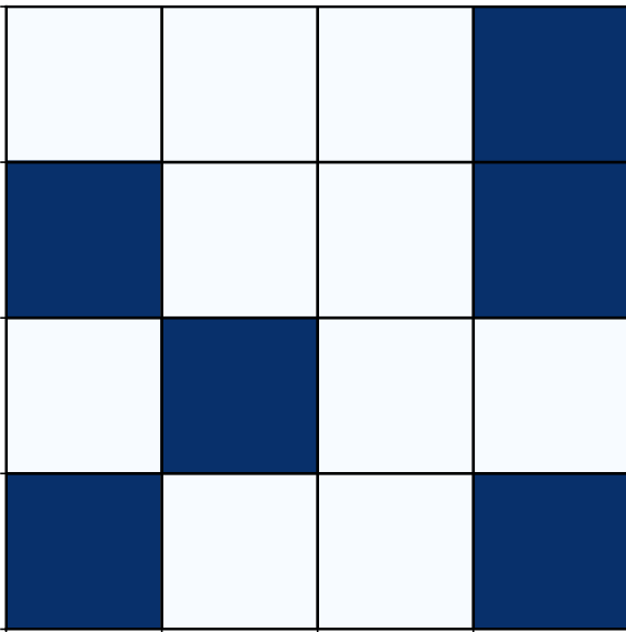
Model 1 | sample 109
