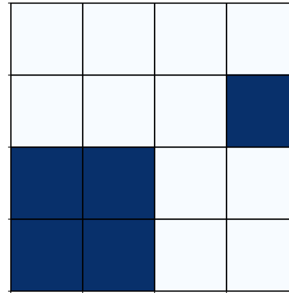
Model 2 | sample 42
