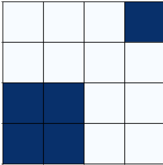
Model 2 | sample 63
