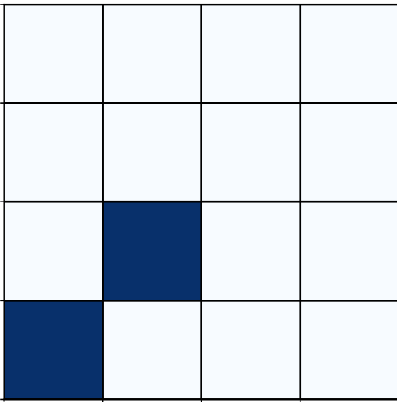
Model 2 | sample 104
