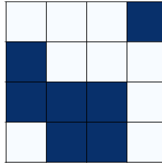
Model 1 | sample 75
