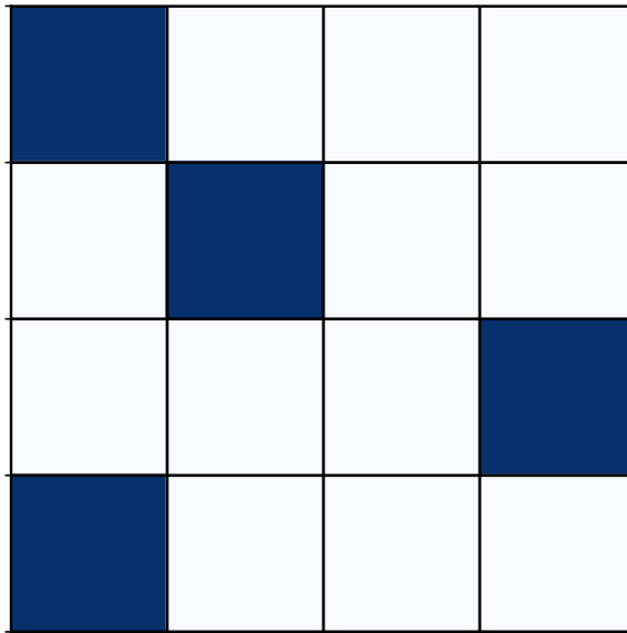
Model 2 | sample 63
