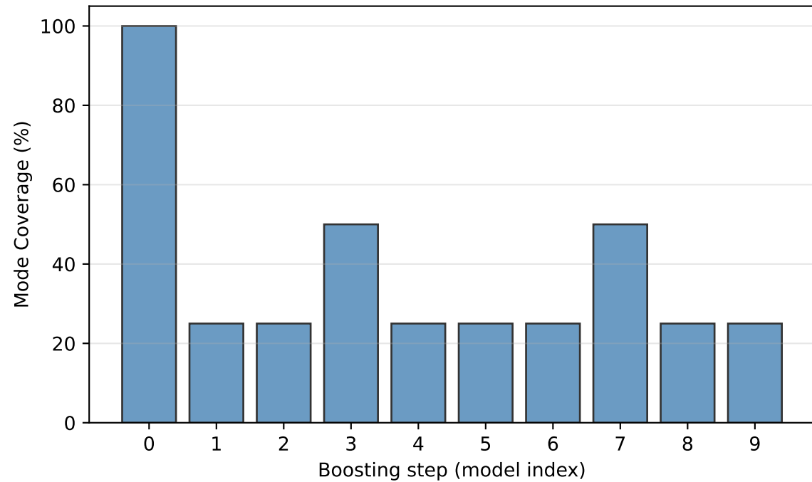
Hamming Balls: Mode Coverage
