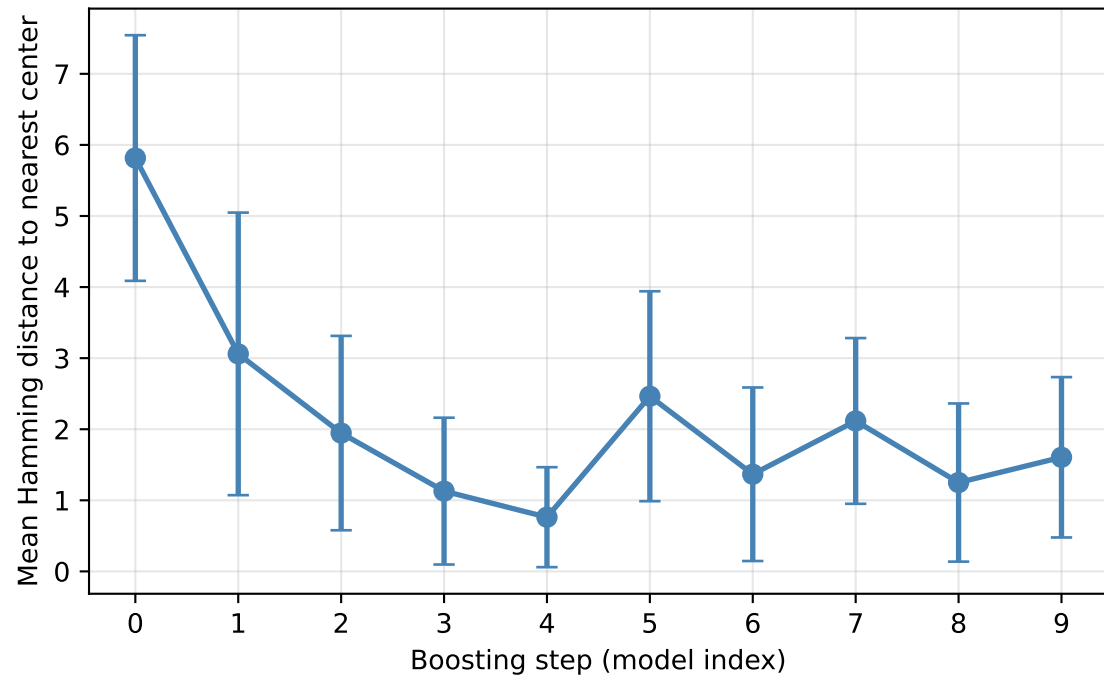
Hamming Balls: Proximity to Centers
