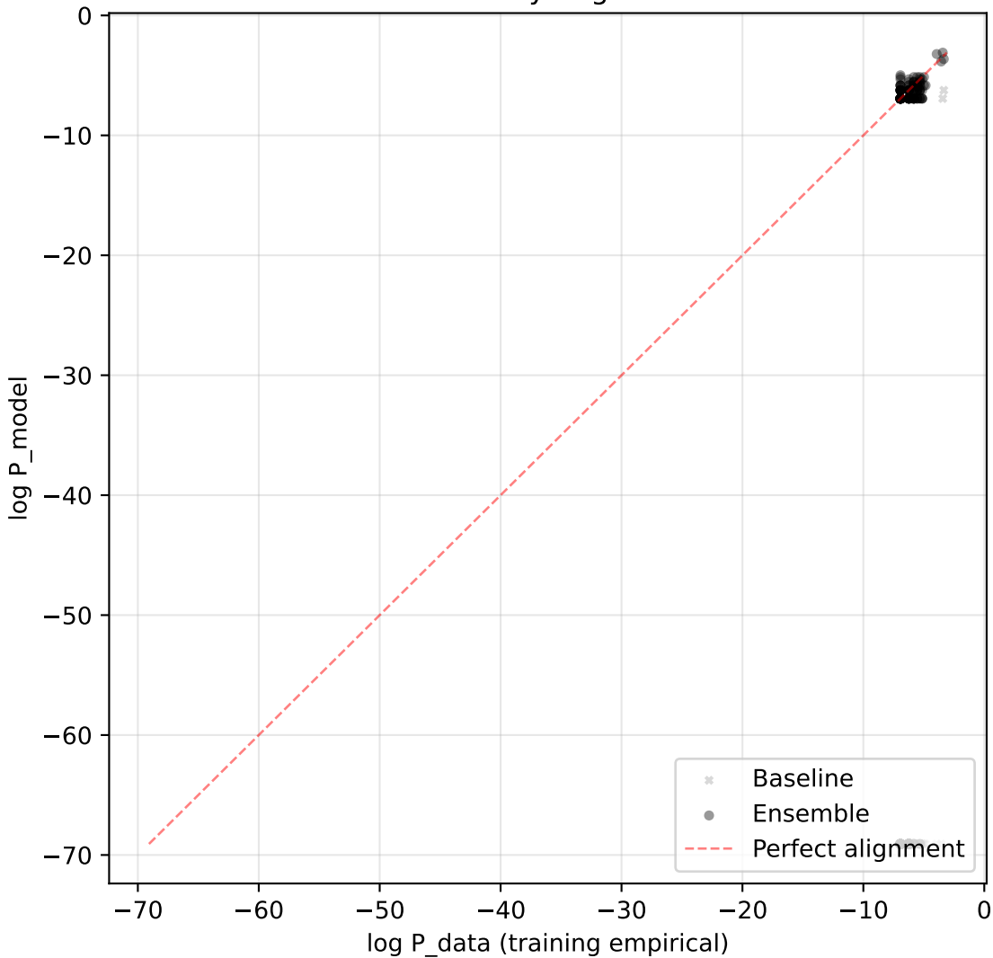
Probability Alignment
