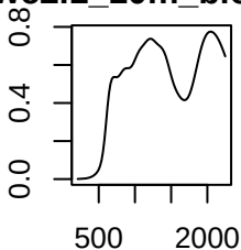
wc2.1_10m_bio_12
