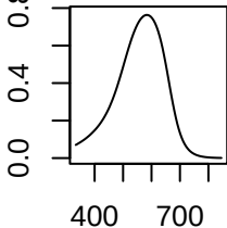
wc2.1_10m_bio_4
