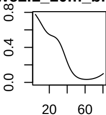
wc2.1_10m_bio_15
