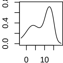
wc2.1_10m_bio_1
