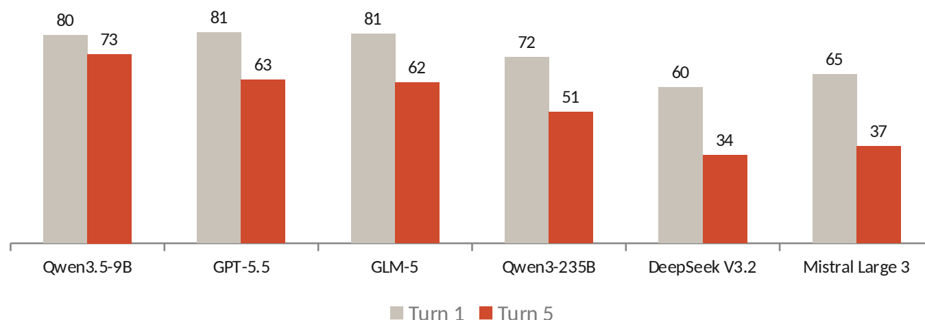
SciFact accuracy, first turn against last (%)
