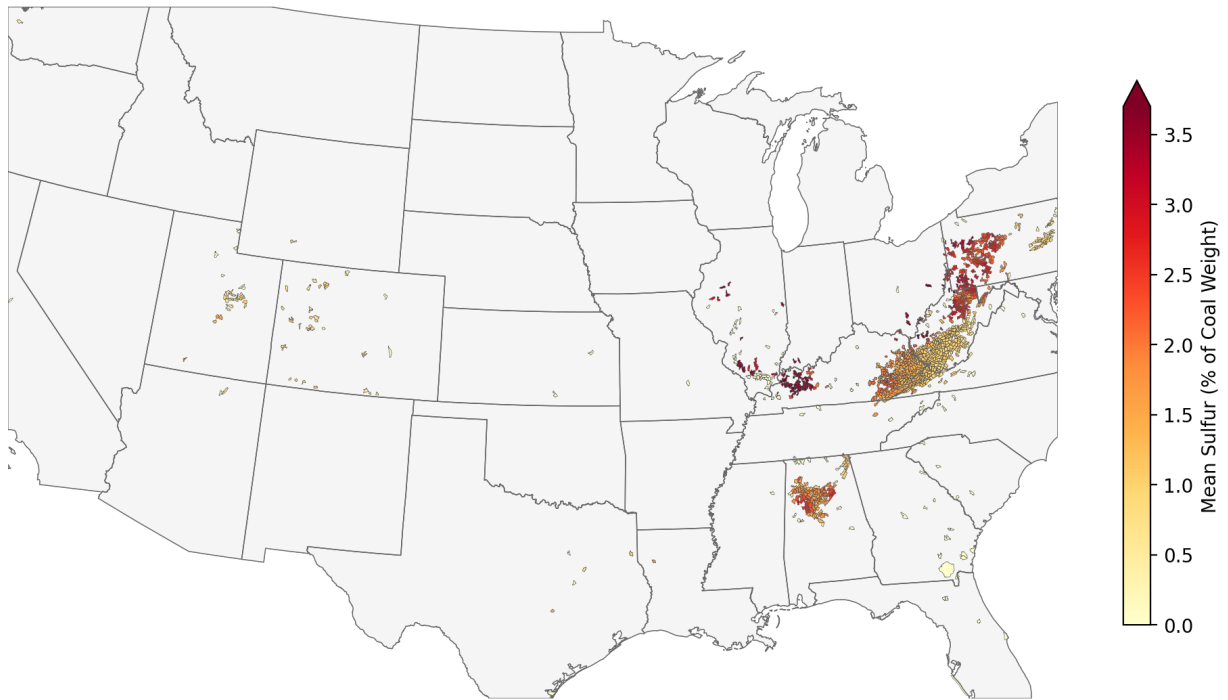
Figure 3: Shading indicates the mean sulfur content of coal, as a percentage of coal weight, for HUC12 watersheds containing an active coal mine. Values are capped at the 95th percentile; watersheds above this threshold appear in the darkest shade, marked by the arrow on the color scale.
