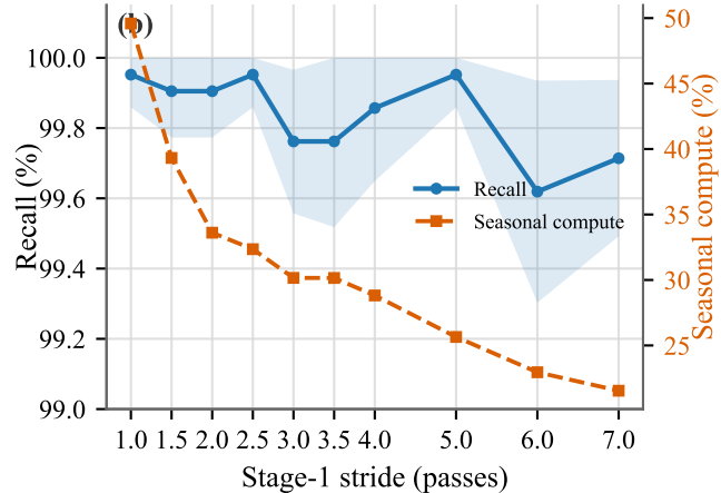
Sparse screening cadence
