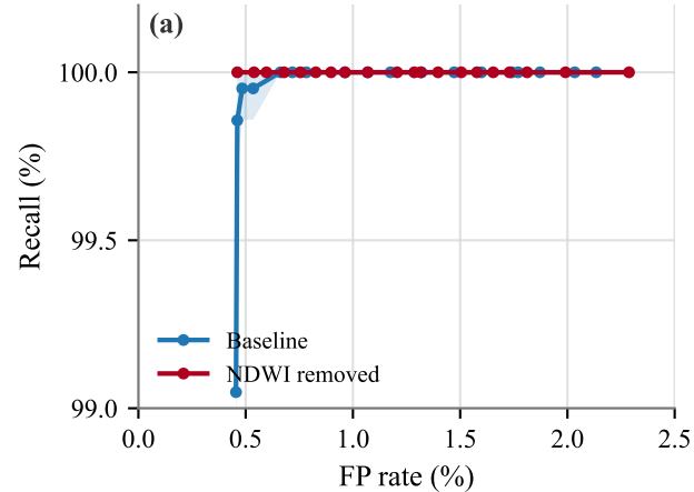
CSC threshold sweep (operating regime)
