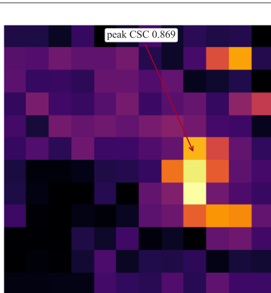
(a) Peak CSC field, Westlands 2014
