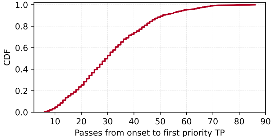
Empirical CDF
