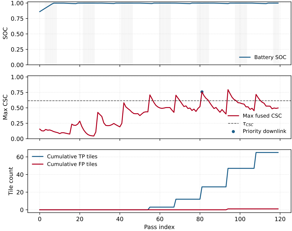
Figure 4: Single-seed synthetic trajectory (seed 0). Battery SOC evolves under the simplified energy model (Table 2); max CSC crosses \tau_{CSC} intermittently, and priority downlink occurs only when a contact window and belief gate coincide.
