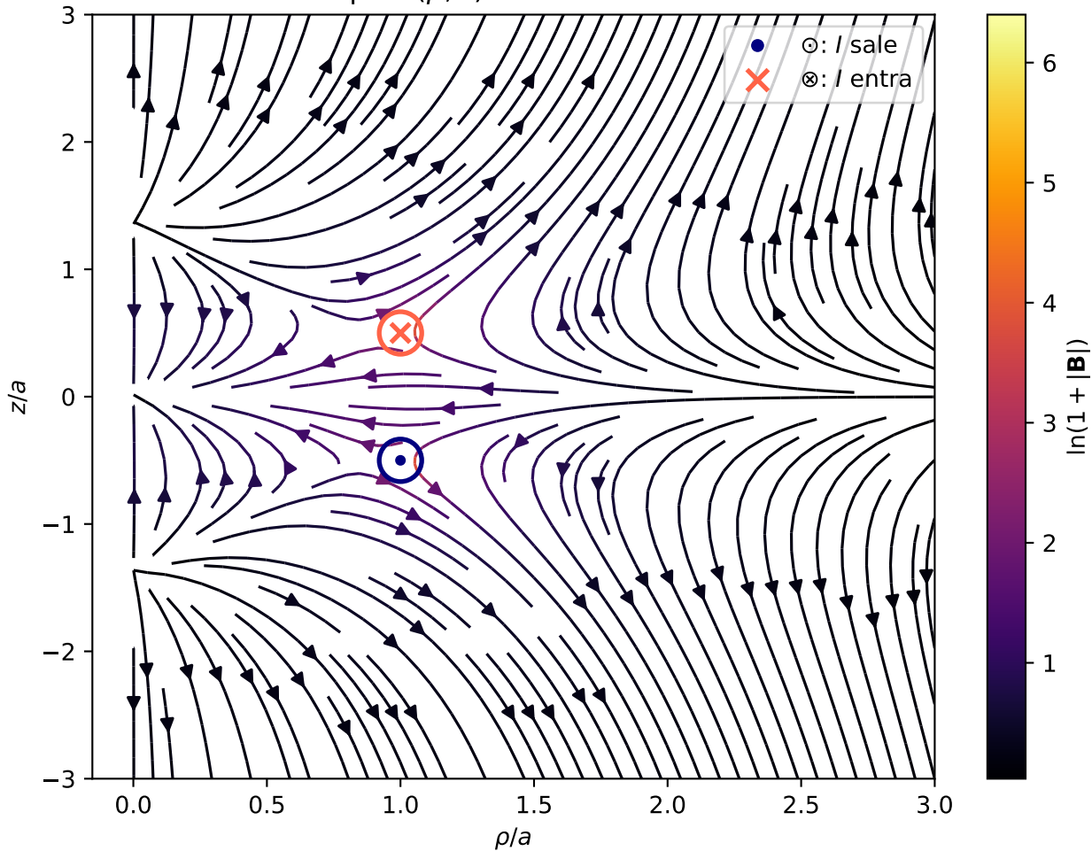
Campo \mathbf{B}(\rho, z) — Anti-Helmholtz
