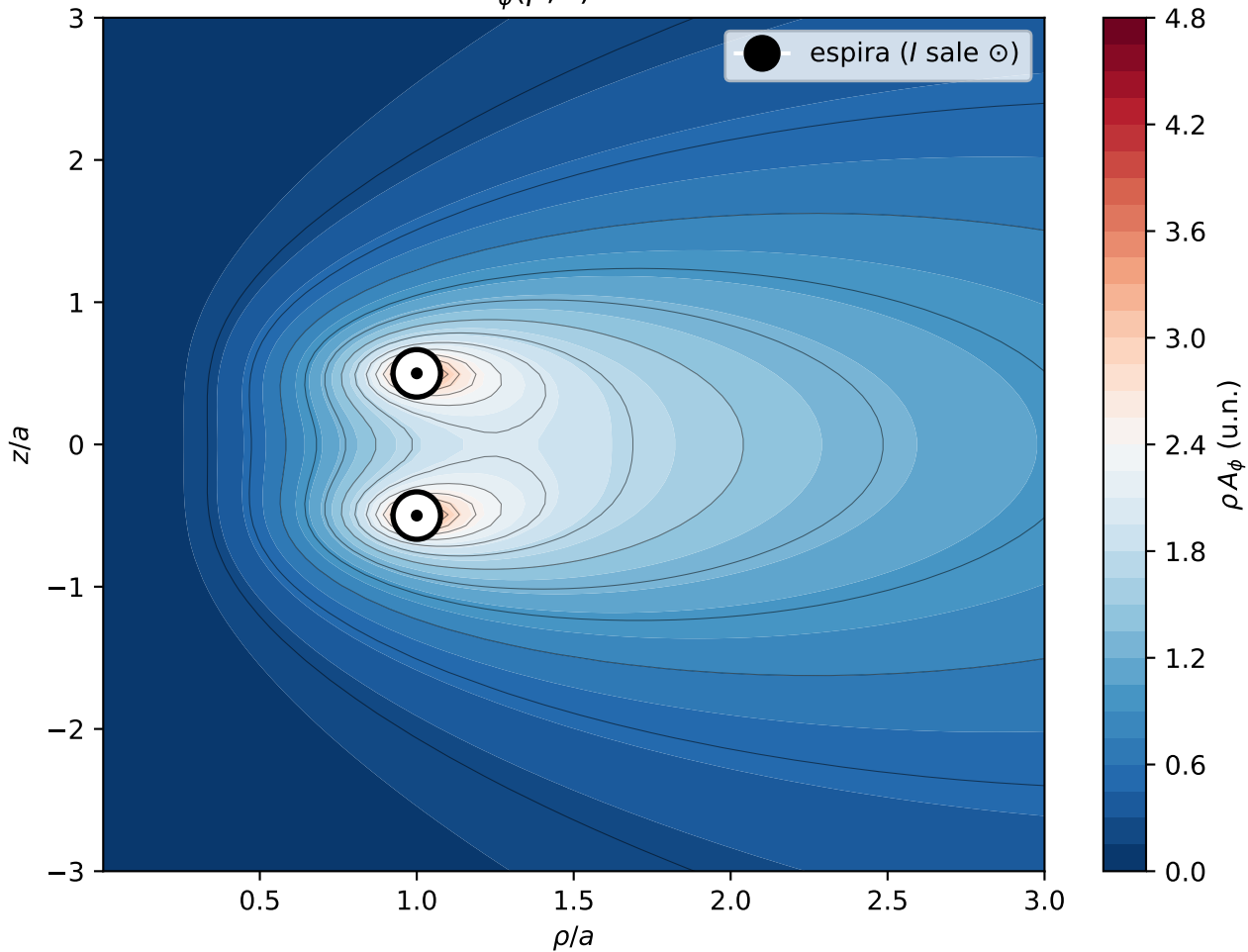
Potential vectorial A_\phi(\rho, z) — Bobina de Helmholtz
