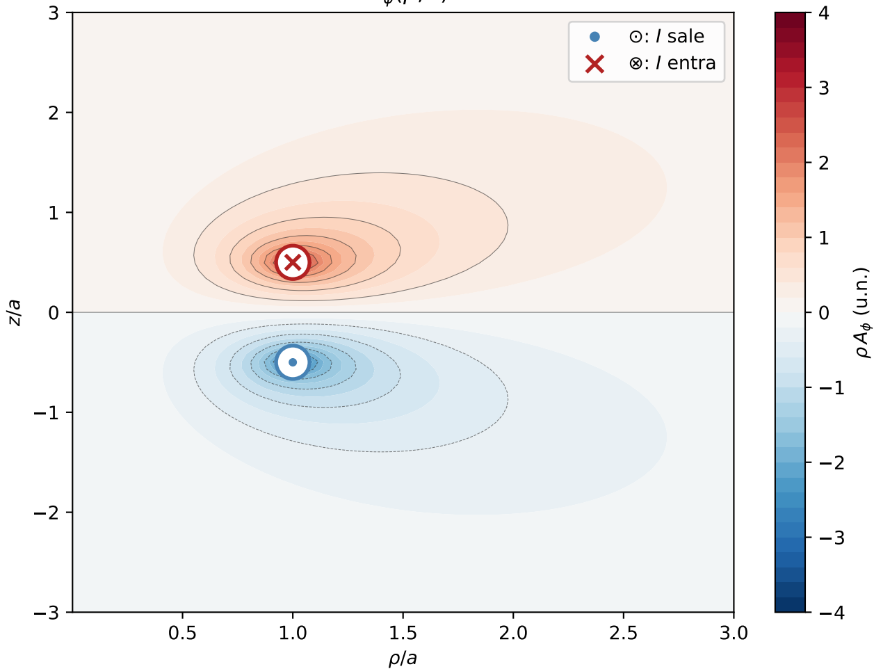
Potencial vectorial A_\phi(\rho, z) — Anti-Helmholtz
