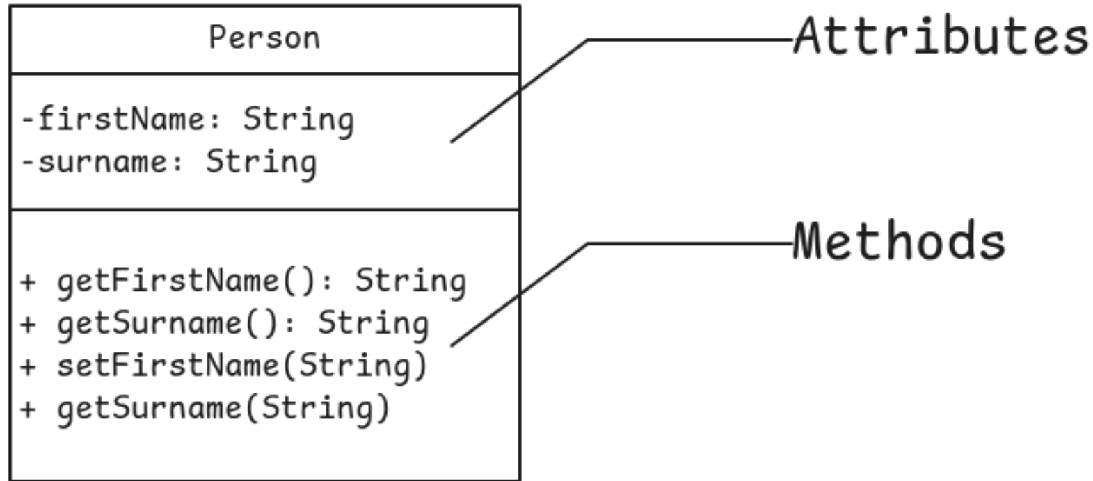
Figure 2: UML Class Diagram
