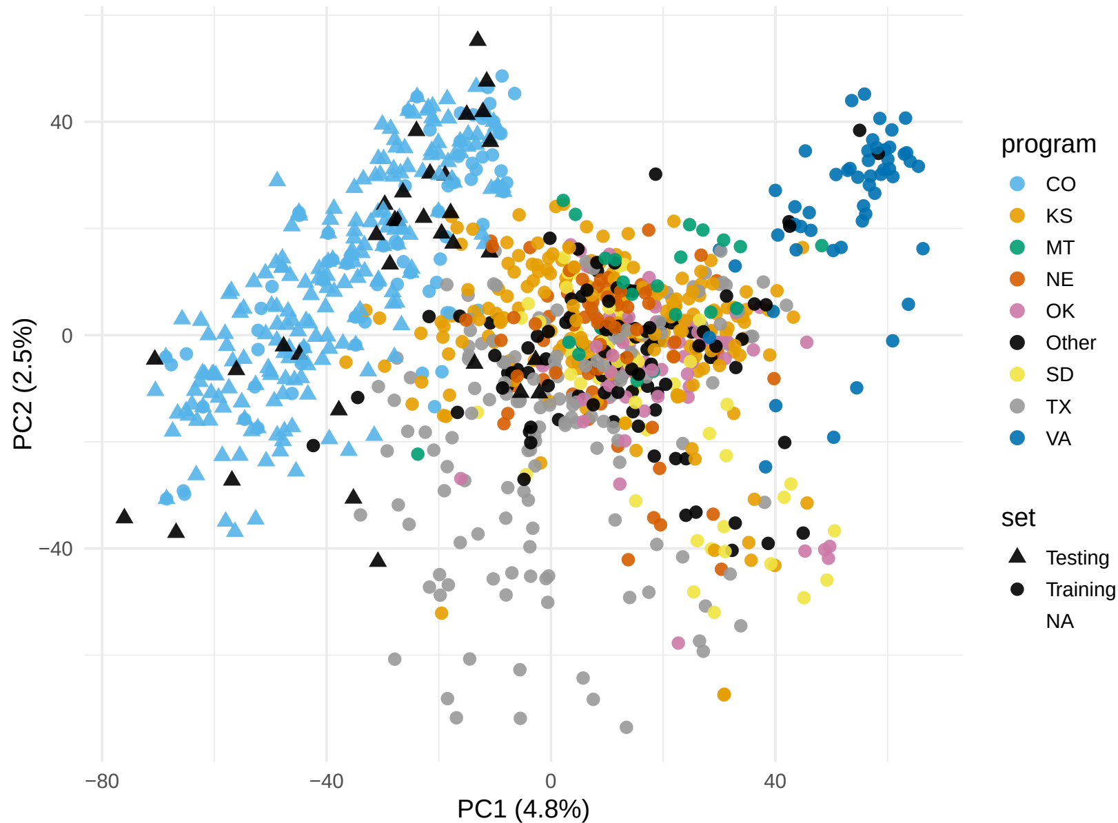
PCA of Genotypes by Program (Color) and Set (Shape)
