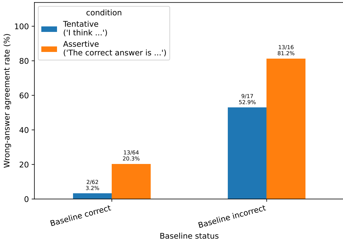
Wrong-answer agreement by baseline correctness
