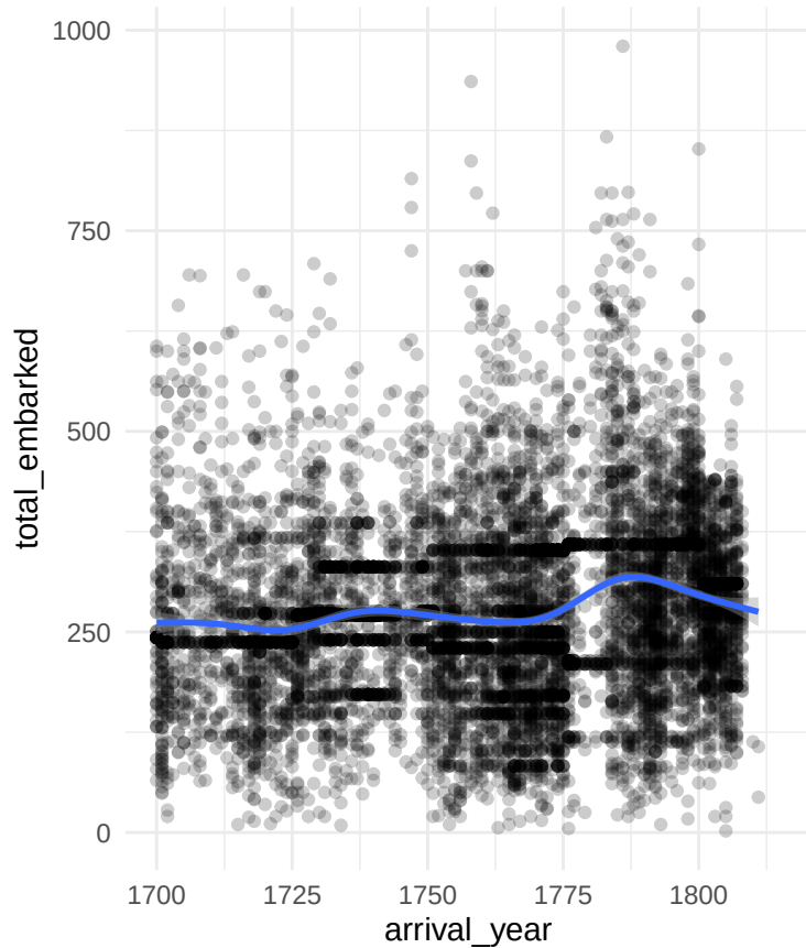
scale_x_continuous(limits=)
