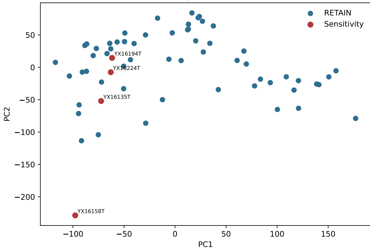
PCA on filtered log2(normalized count + 1)
