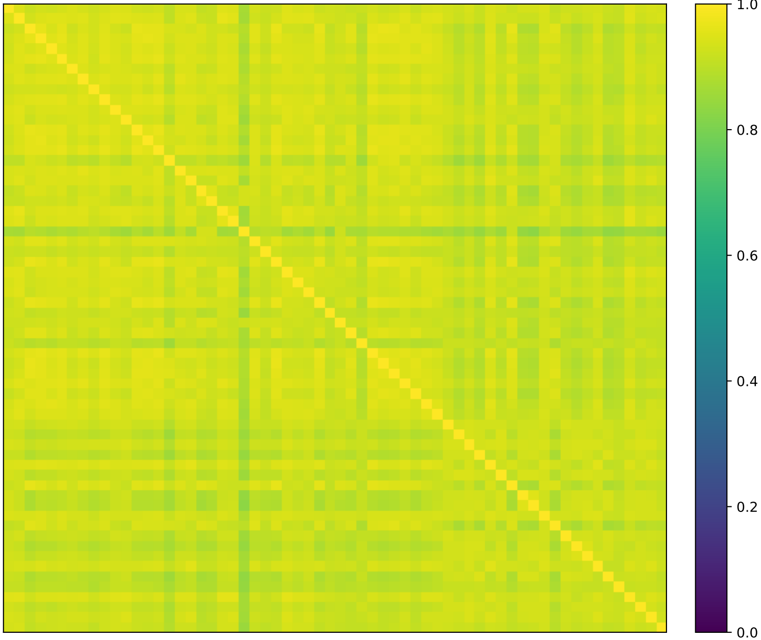
Sample correlation, filtered log2 matrix
