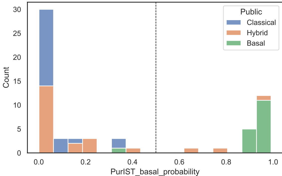
Assignment Confidence
