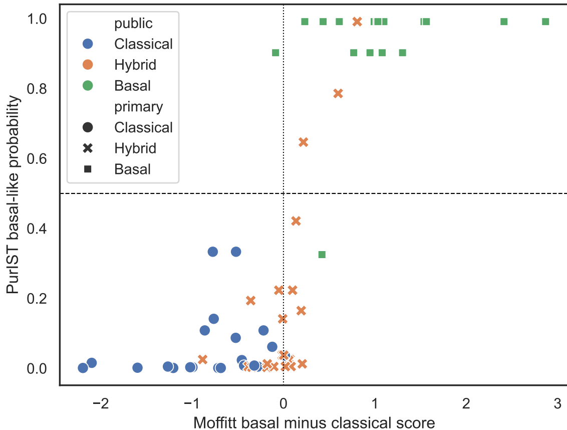
Basal-Classical Axis
