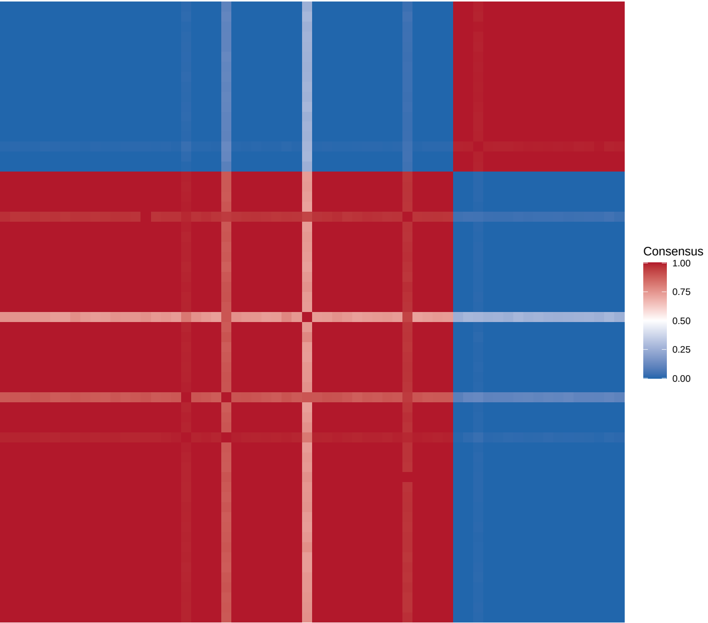
Primary CSY consensus matrix, K=2
