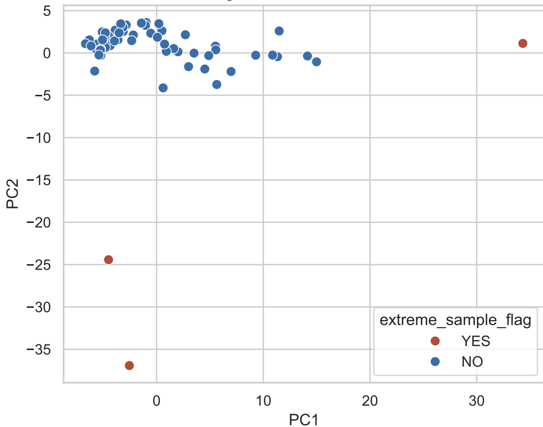
PCA of log10 Relative Genus Abundance
