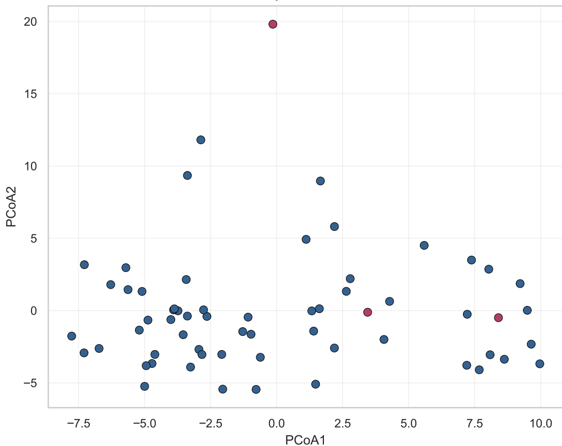
Primary Aitchison PCoA
