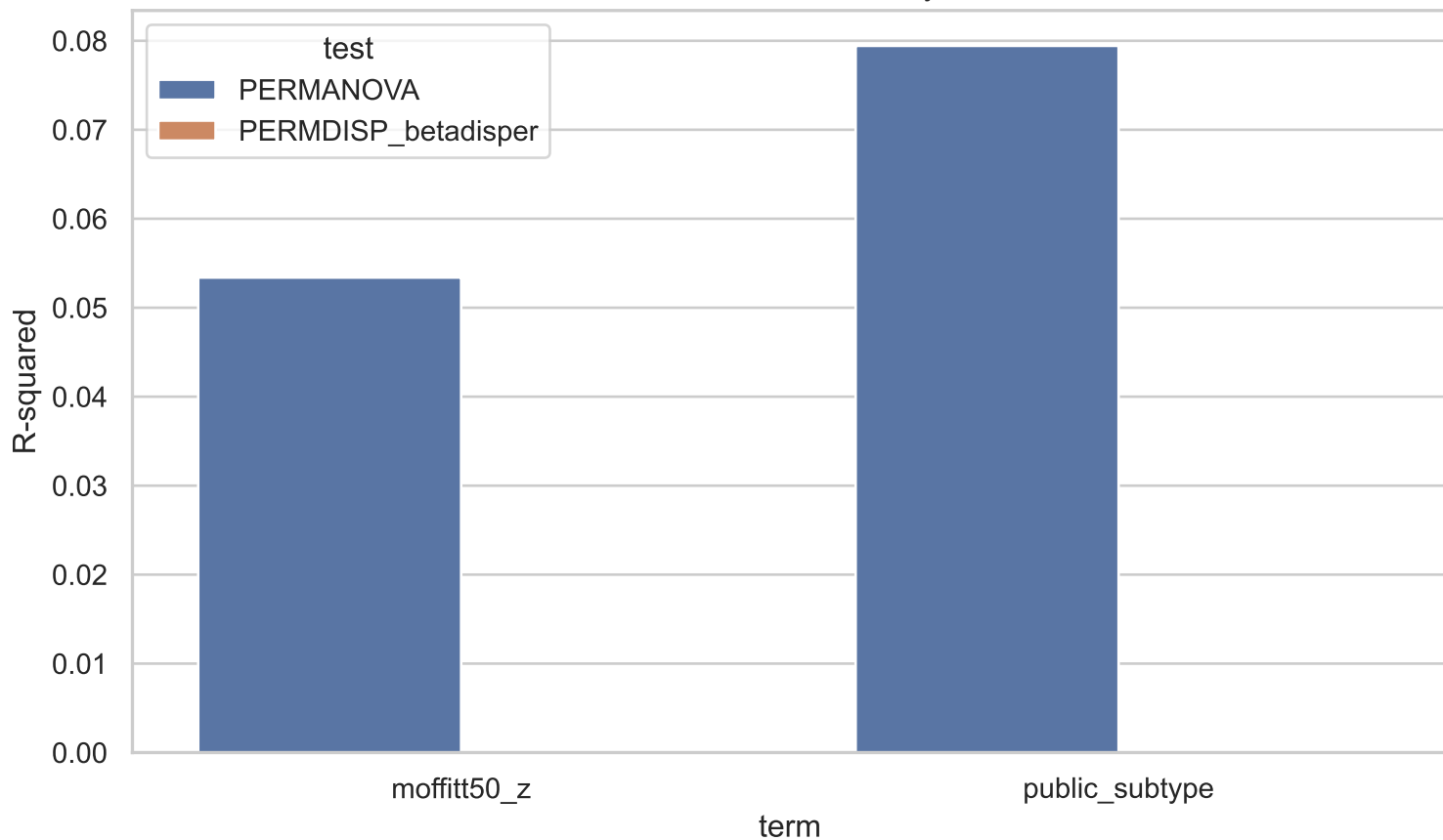
Phase 7B Global Community Effects
