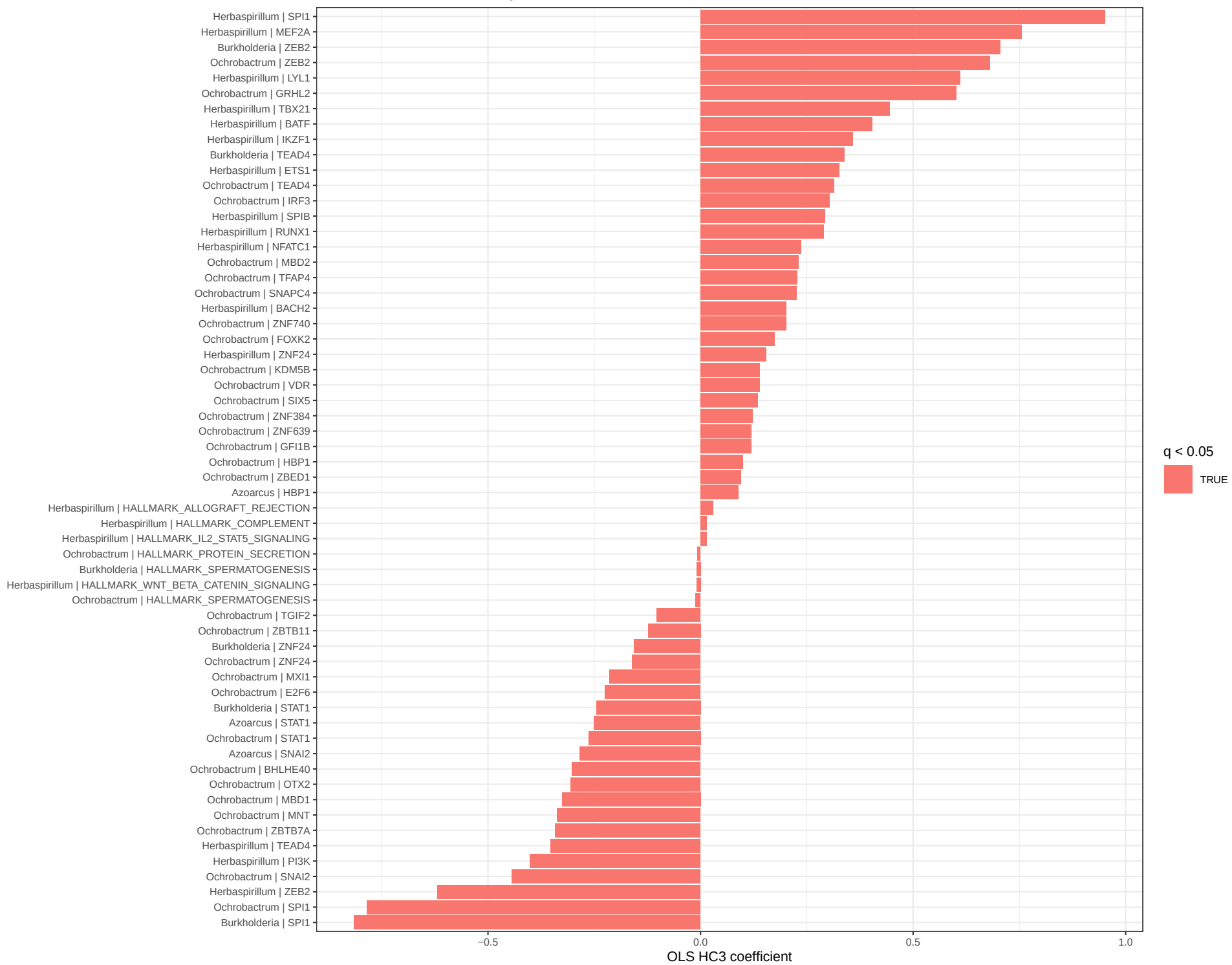
Phase 8B rCLR Sensitivity
