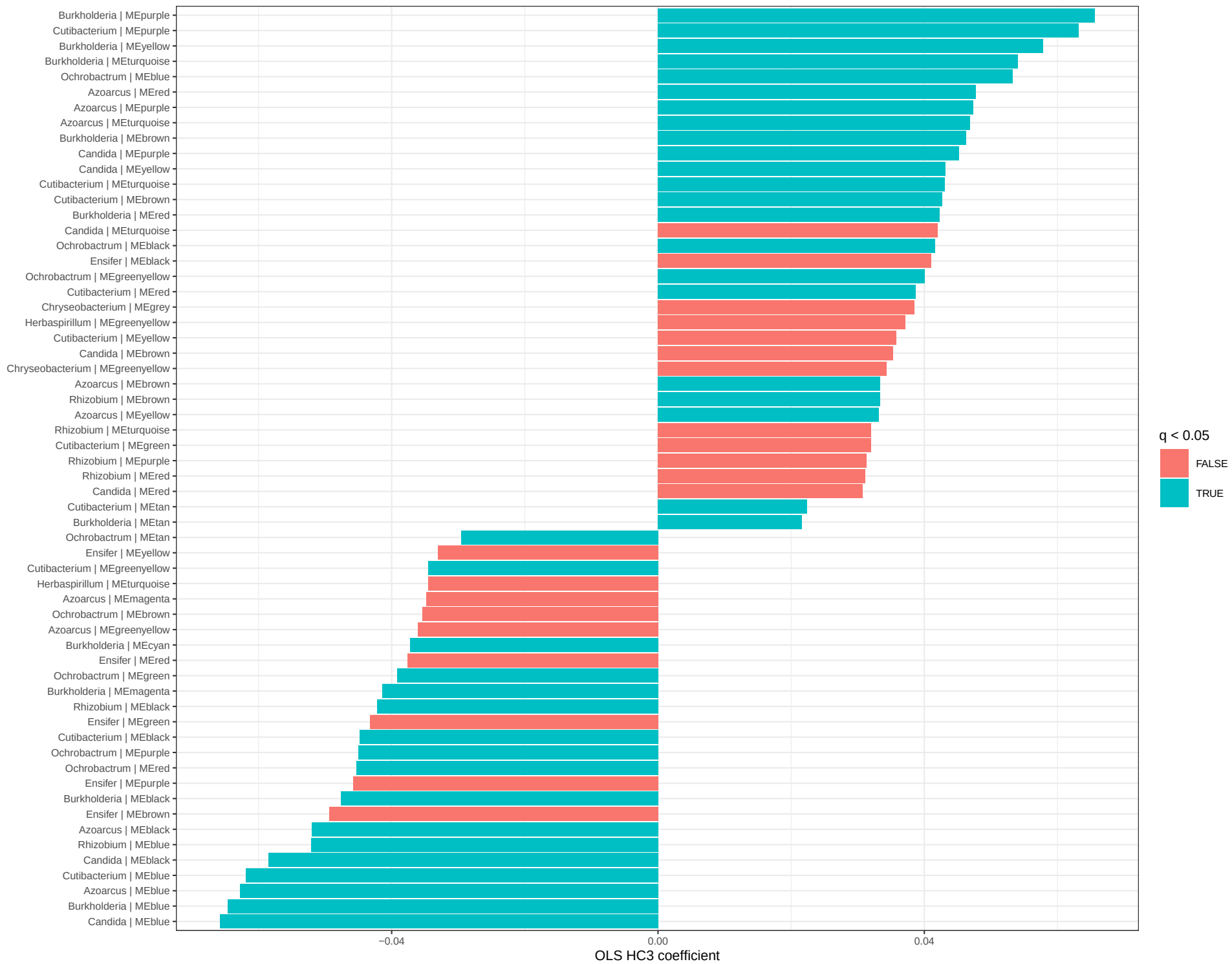
Phase 8B WGCNA Module Associations
