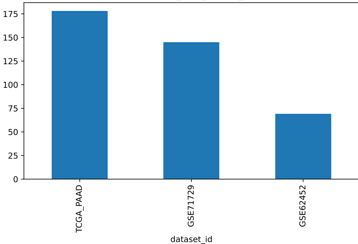
phase9b1_bulk_cohort_qc
